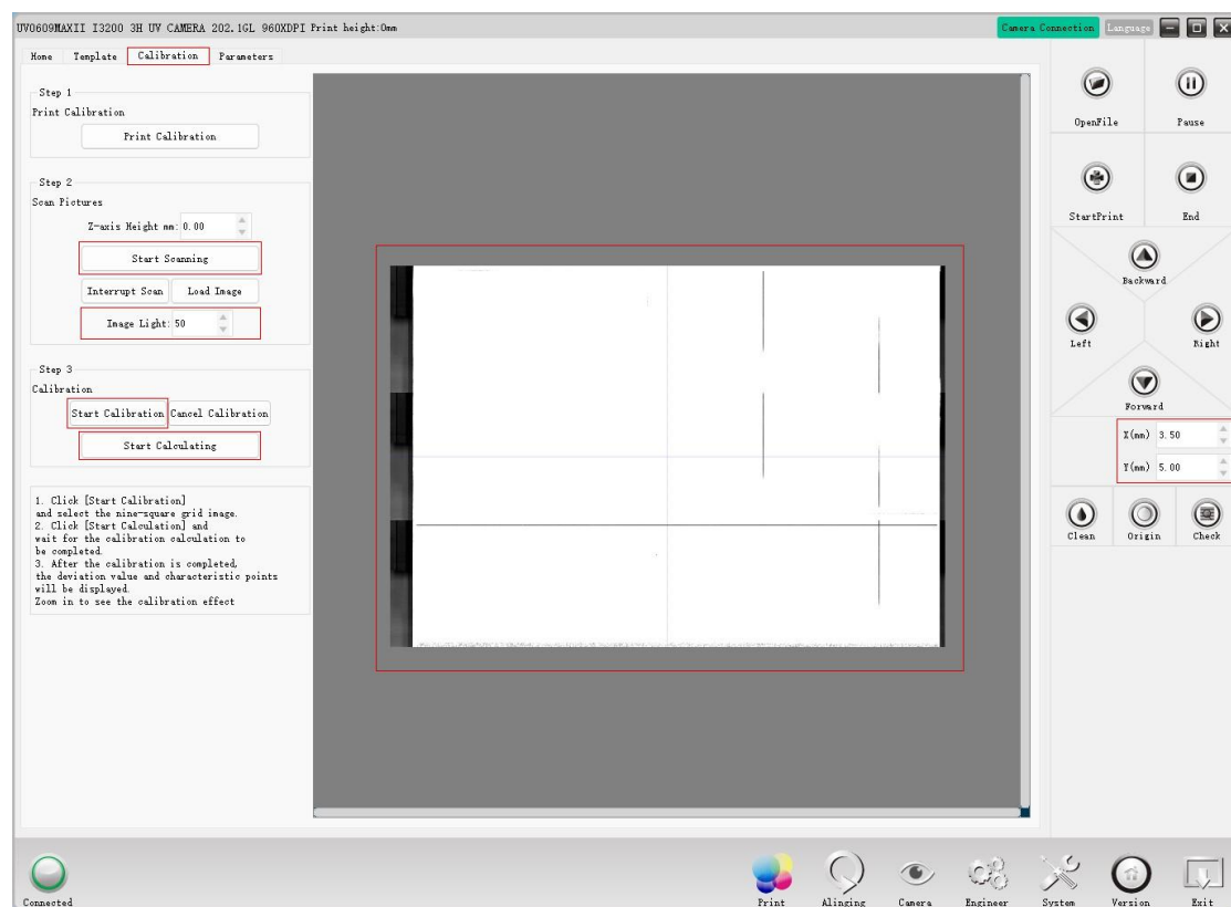
5-1 Camera calibration
